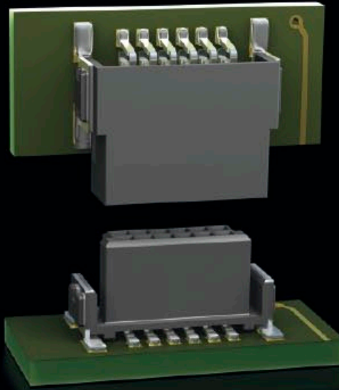
Mother-to-Daughtercard
